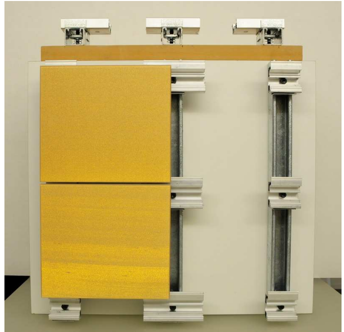
Kuwait National Museum Treasury – model of internal wall cladding system developed by 3form for Varia Ecoresin, design Studio A London
