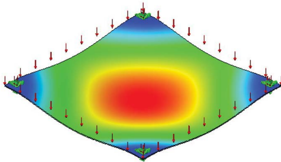
Figure 5. Point-support deflection diagram
