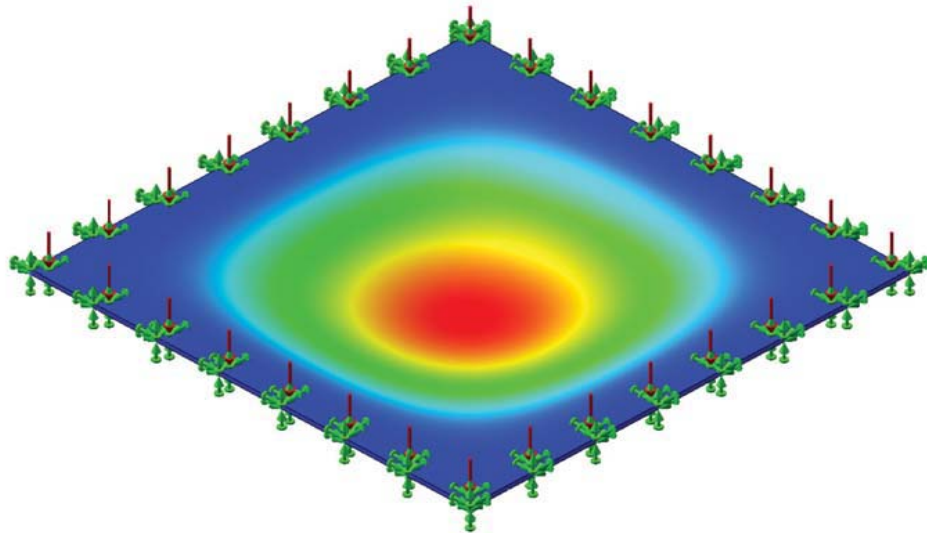
Figure 1. Fully framed support deflection diagram
